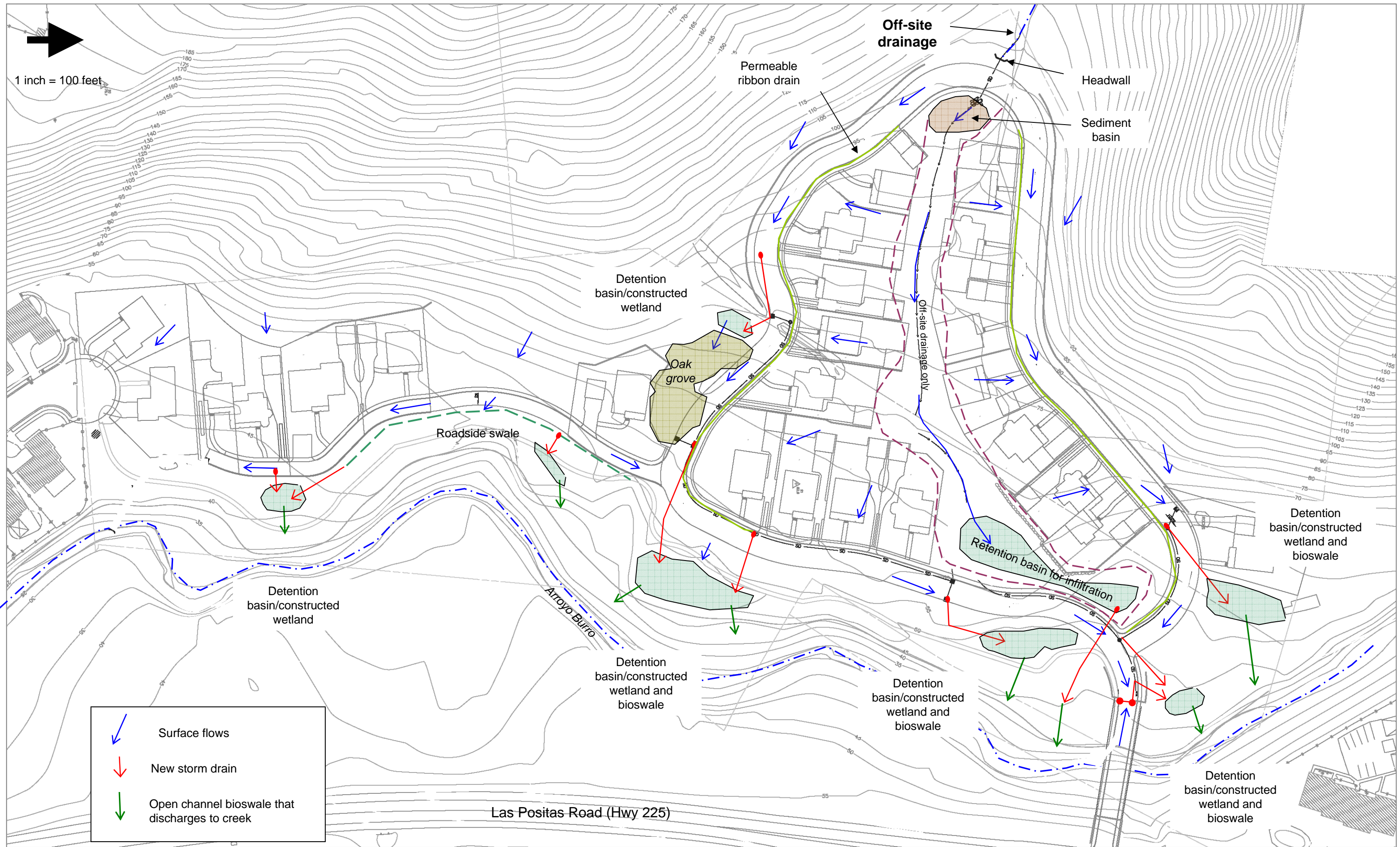
Figure 4-6. Alternative Drainage and Stormwater Treatment Plan
