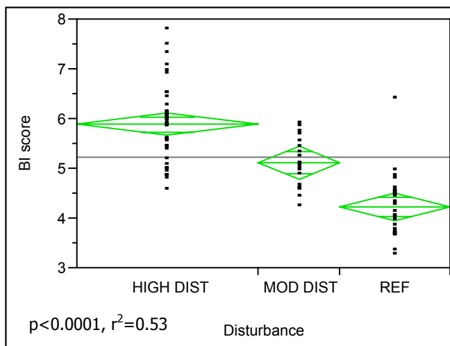
Figure 7: ANOVA Comparison of Biotic Index Score at UNDIST (i.e., REF), MOD DIST, and HIGH DIST Reaches
