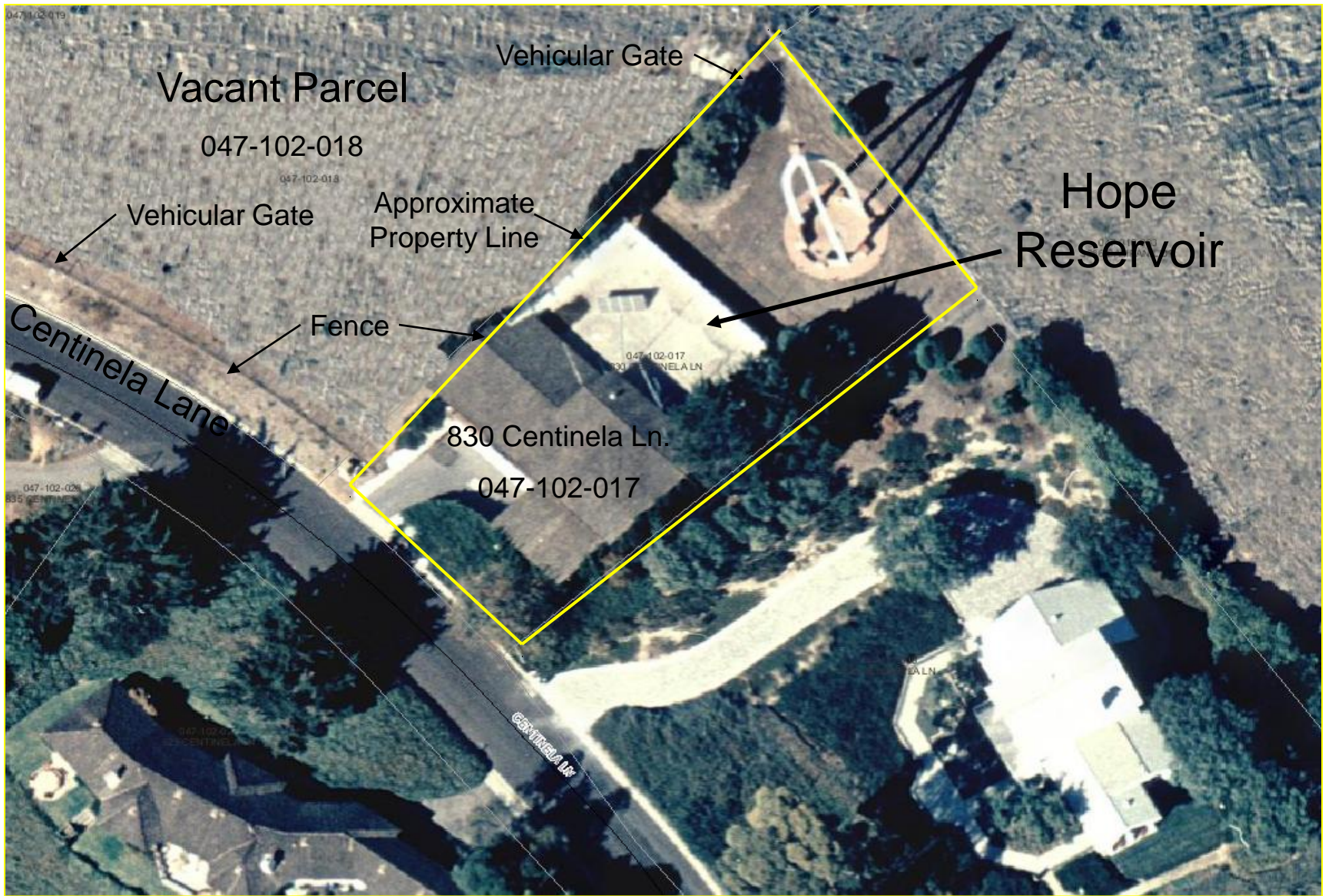
Hope Reservoir Site Plan
