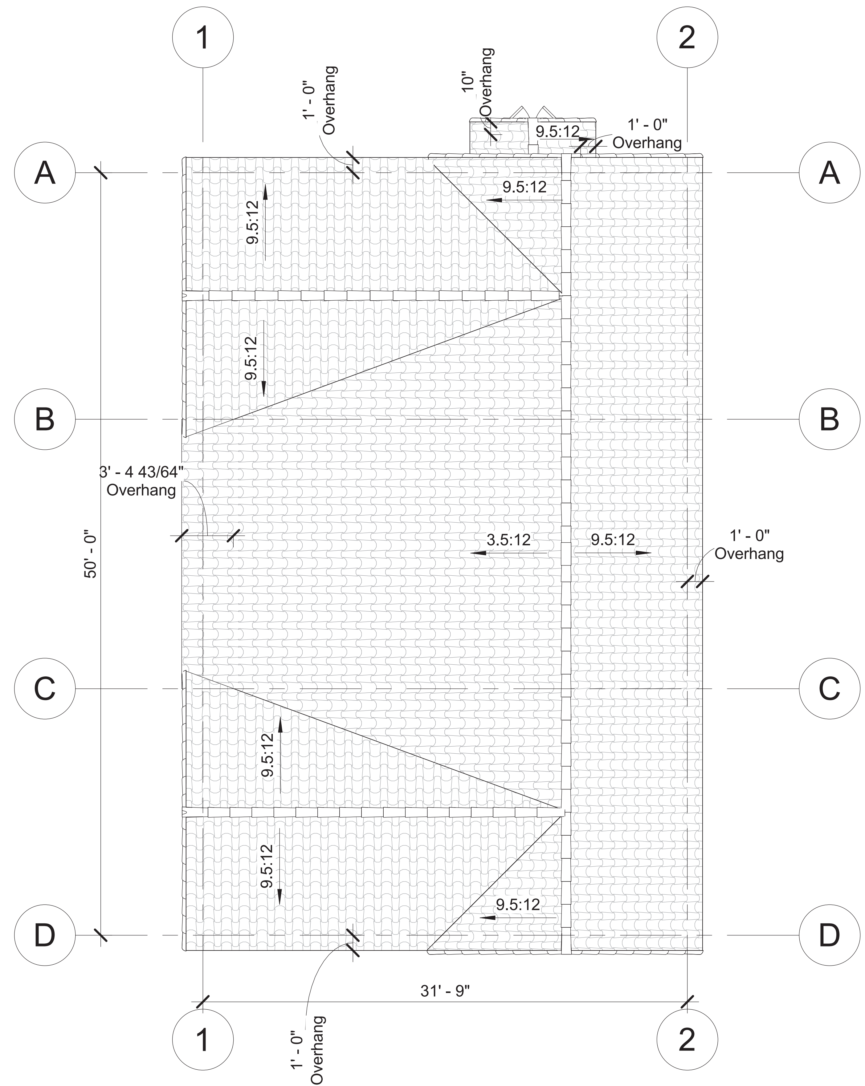
1 WELCOME HOUSE ROOF PLAN 1/4" = 1'-0"
