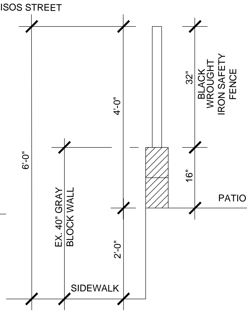
PROPOSED ELEVATION A - A SCALE: 1" = 1'-0"
