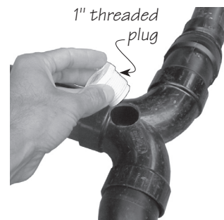
A double ell retrofitted with inspection access. The access is sealed with a threaded plug.
