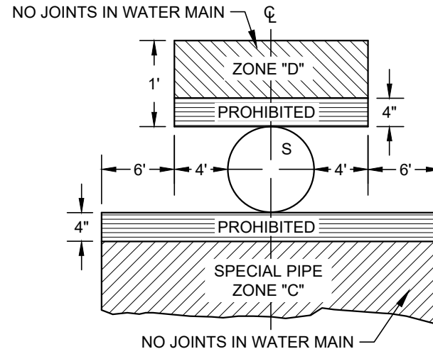
PERPENDICULAR CONSTRUCTION (CROSSINGS)
