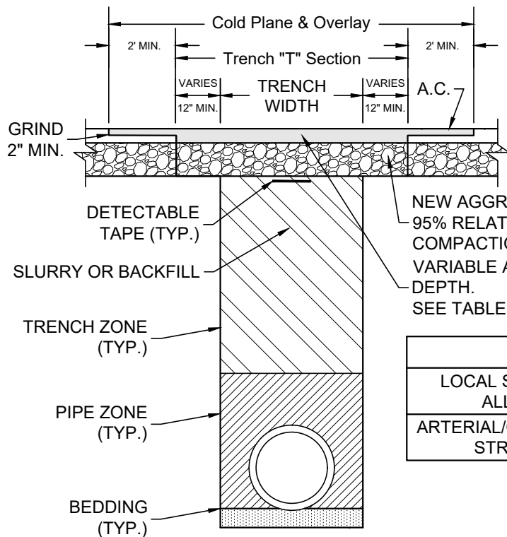
A.C. OVER AGGREGATE BASE OPTION 1
