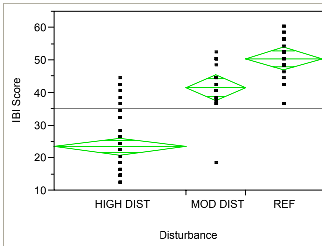
Figure 9: ANOVA Comparison of IBI Score at UNDIST (i.e., REF), MOD DIST, and HIGH DIST Reaches
