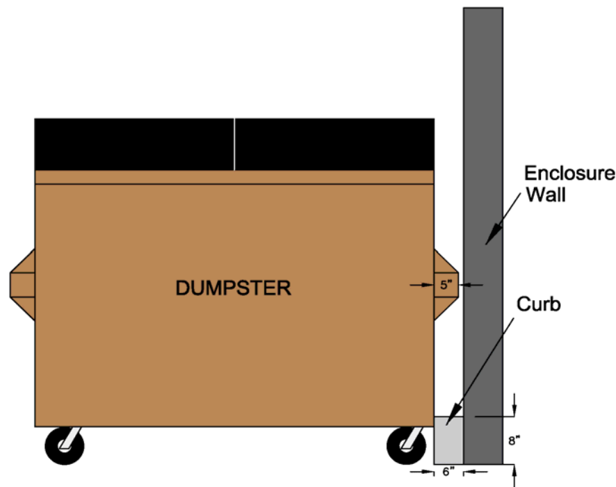
Figure 3: Curb Detail
