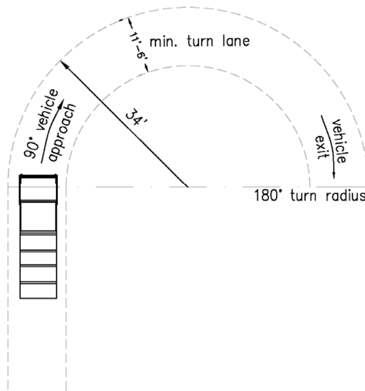
Figure 2: Truck Turning Radius
